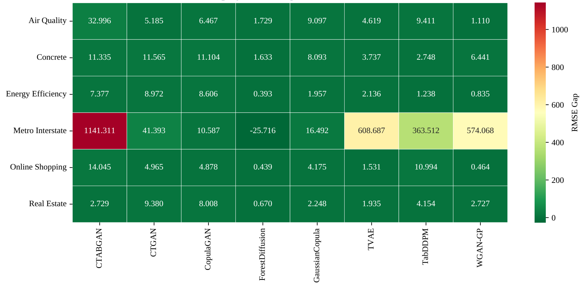
RMSE Gap by dataset × generator (10-seed mean)
